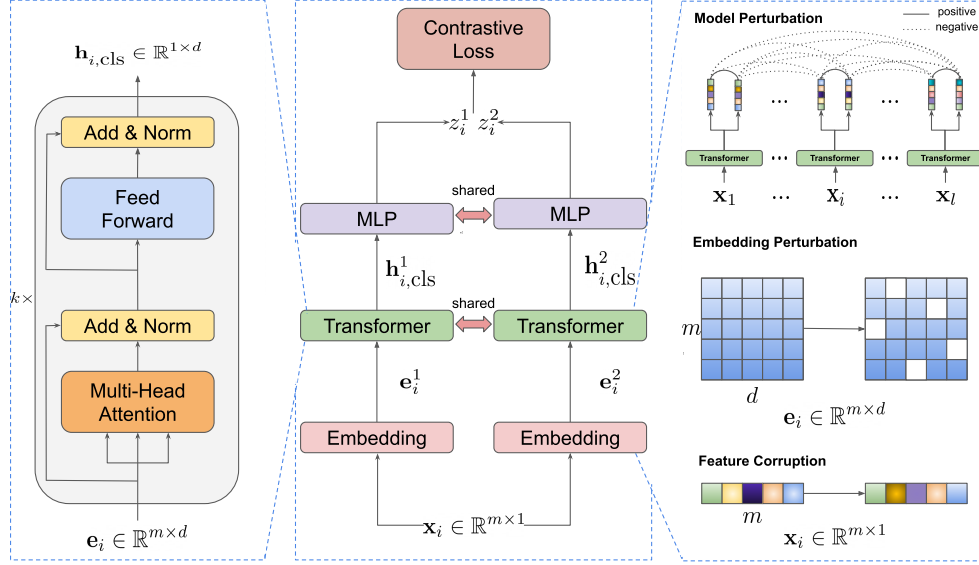
Figure 1: Model architecture diagram for our contrastive learning approach. For each input instance \mathbf{x}_i we sample two augmentation operators and apply them to \mathbf{x}_i as it is passed through an embedding layer and k Transformer blocks, resulting in two augmented view representations \mathbf{h}_i^1 and \mathbf{h}_i^2 . The views are then passed through an MLP to get the embeddings \mathbf{z}_i^1 and \mathbf{z}_i^2 which are treated as a positive pair in the contrastive loss and pushed together; all other views in the batch are treated as negatives and pushed away from (\mathbf{z}_i^1, \mathbf{z}_i^2) .
